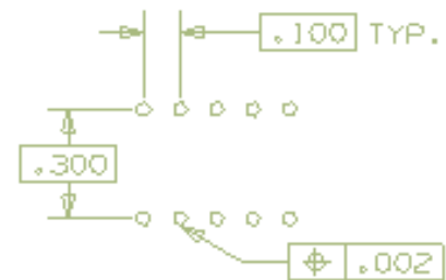
RECOMMENDED PC HOLE PATTERN
